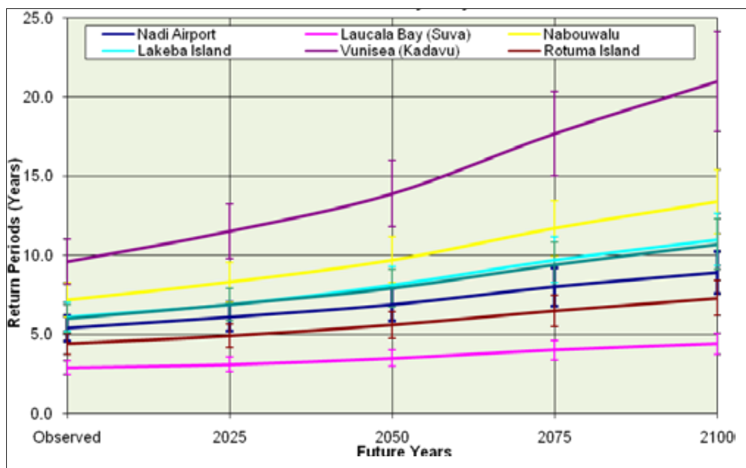
Figure A1- 7: Projections for daily maximum rainfall of 200 mm at various locations in Fiji projected to 2100 Data source: Fiji Meteorological Services 2011
