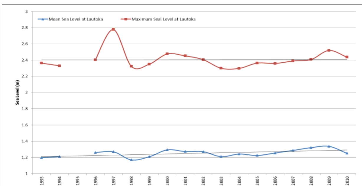
Figure A1-5: Trends in mean and maximum sea levels at Lautoka tide gauge, 1993–2010
