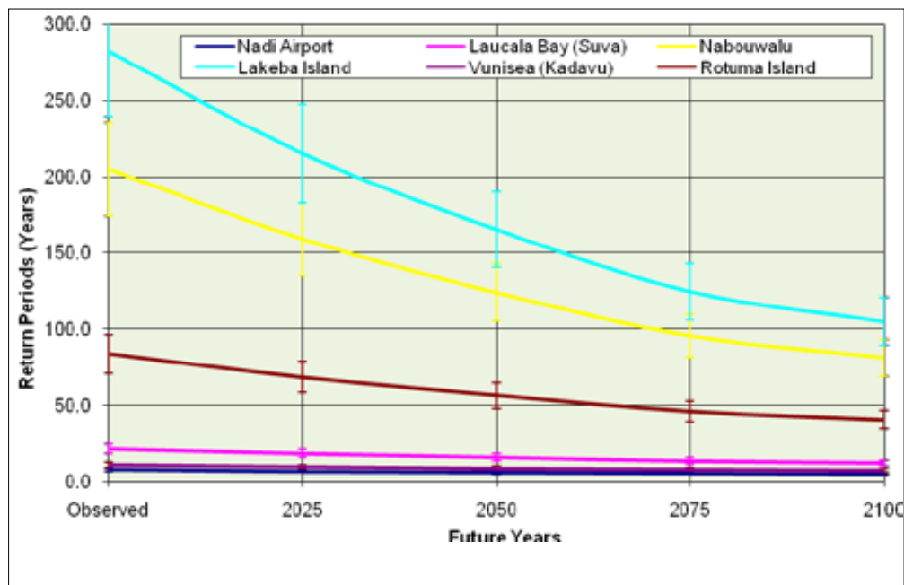
Figure A1-10: Climate risk of maximum winds of 80 knots at various locations in Fiji projected to 2100 Data source: Fiji Meteorological Services 2011
