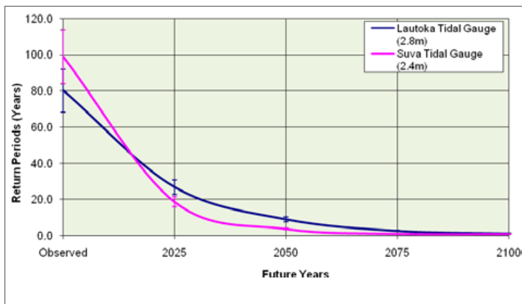
Figure A1-11: Climate risk of maximum sea level at various locations in Fiji projected to 2100 Data source: Fiji Meteorological Services 2011
