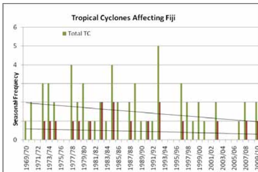
Figure A1-6: Seasonal frequency and hurricane intensity of tropical cyclones affecting Fiji from 1969/70 to 2009/10.
