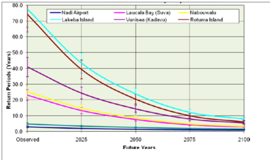
Figure A1-8: Projections for daily maximum temperature of 35°C at various locations in Fiji projected to 2100 Data source: Fiji Meteorological Services 2011
