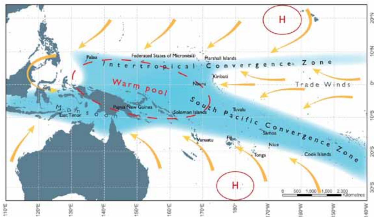
Figure 1. South Pacific Convergence Zone and Inter-Tropical Convergence Zone (Source: Figure ES.2 in Australian Bureau of Meteorology and CSIRO 2011, Climate Change in the Pacific: Scientific Assessment and New Research. Volume 1 Regional. Volume 2 Country Reports )
