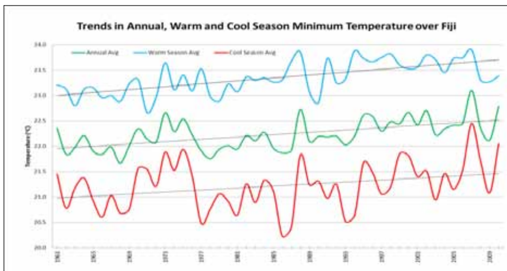
Figure A1-2: Inter-annual and seasonal variation in minimum temperature over Fiji, 1961 to 2010 Data source: Fiji Meteorological Services 2011
