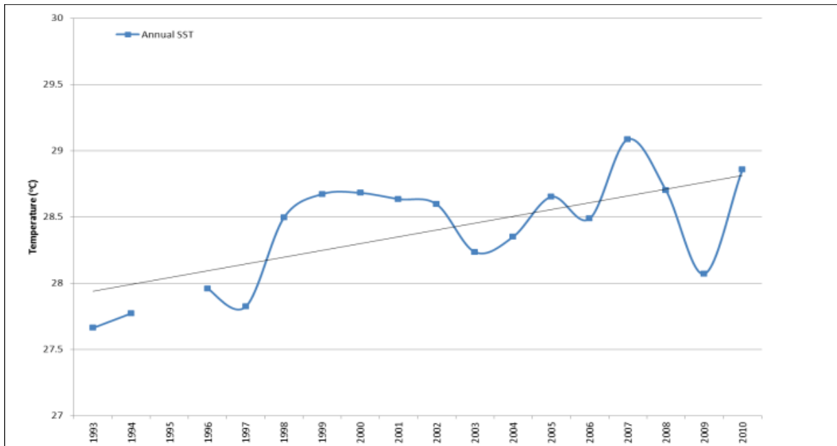
Figure A1-4: Annual sea surface temperature trends at the Lautoka tide gauge, 1993–2010
