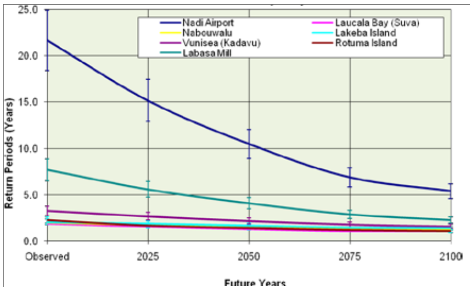
Figure A1-9: Projections for daily minimum temperature of 16°C at various locations in Fiji projected to 2100 Data source: Fiji Meteorological Services 2011
