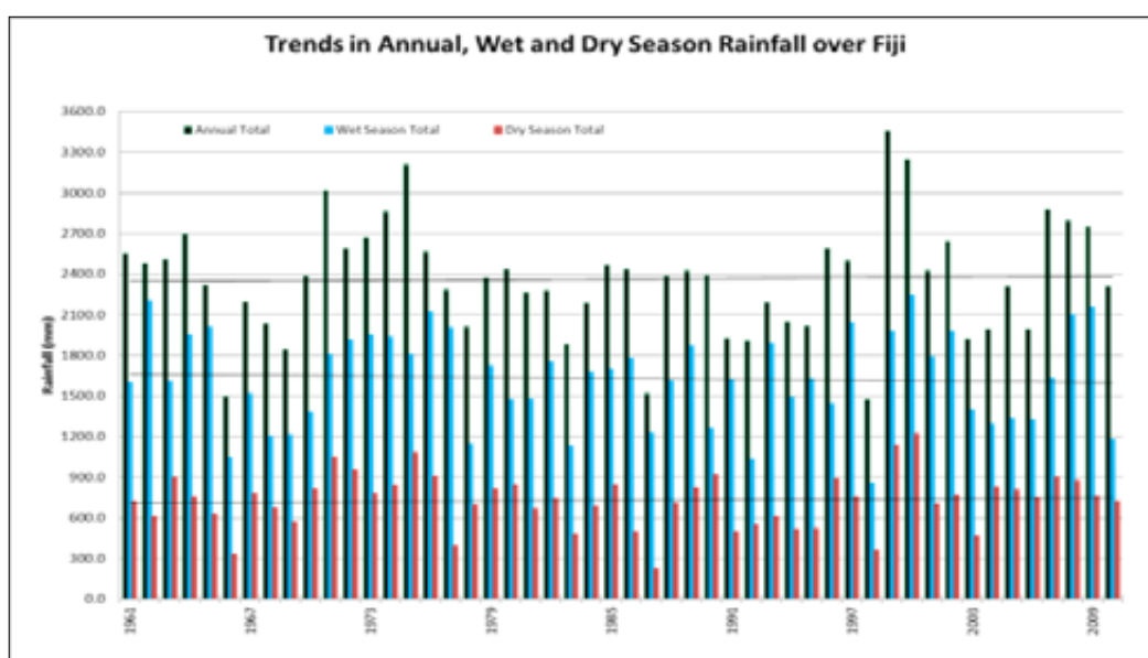
Figure A1-1: High inter-annual variation in annual and seasonal rainfall over Fiji, 1961 to 2010 Data source: Fiji Meteorological Services 2011
