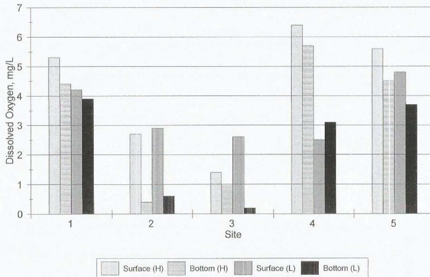
FIGUR E 4. D.O Along Qawa River 30th, May, 1996
