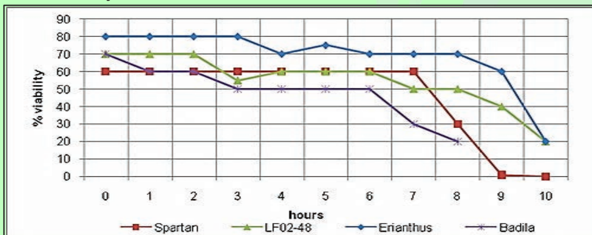
Figure 1: Life span of Erianthus arundinaceus , Saccharum officinarum (Badilla), Spartan and LF02-48 pollen
